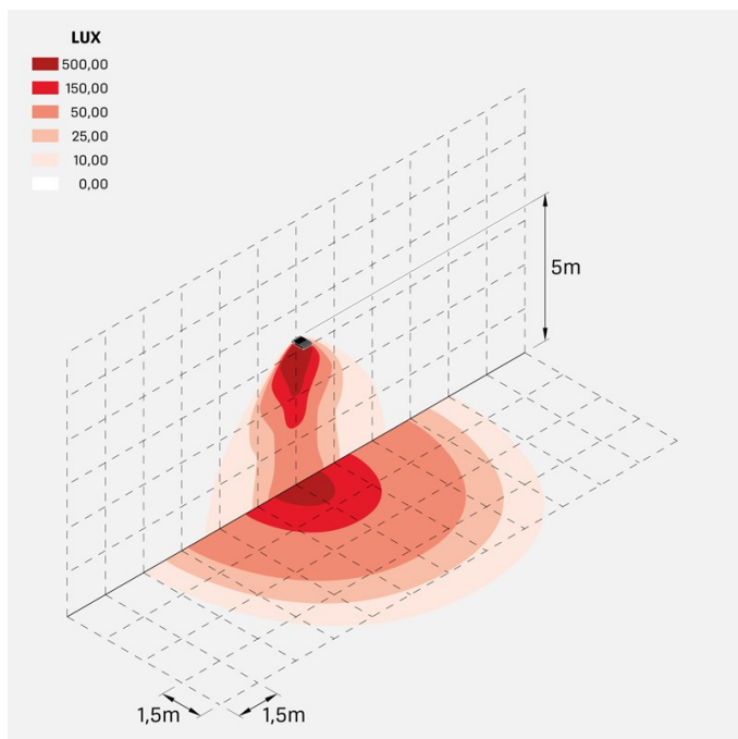
delta2_circular_120W_optic_C1
