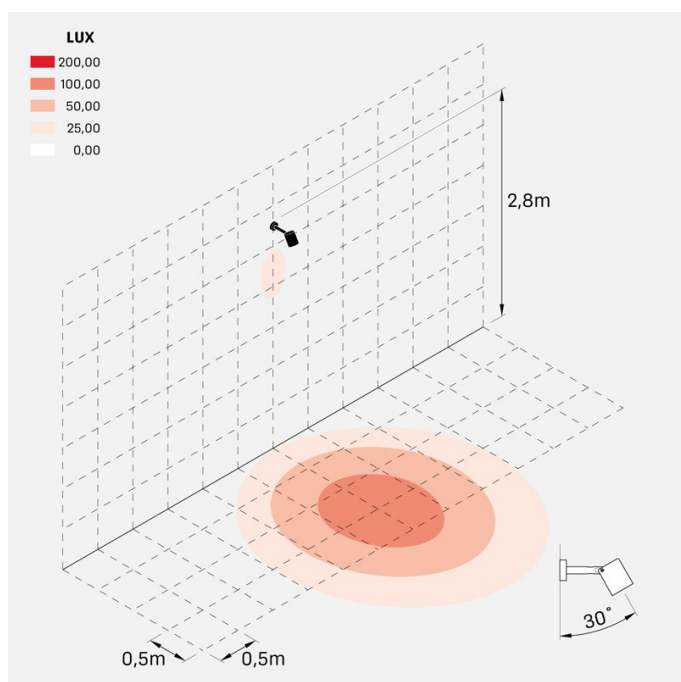
ago_plus_wall_honeycomb_optic_S
