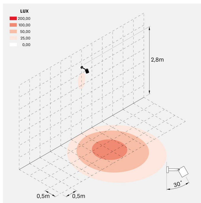
ago_plus_wall_honeycomb_optic_M
